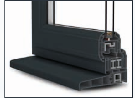
uPVC or aluminium frame windows and doors with thermal breaks and double glazed with 4mm toughened safety glass, argon filled with planitherm coating (see page 28 for further information)
