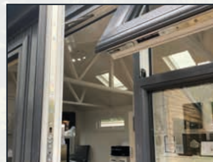
Side casements and top opening vents showing multipoint locking including end shoot bolts
