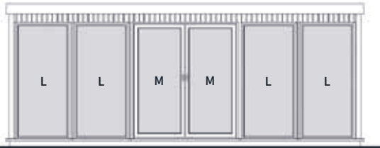
6.10m (20') front with 1.80m double doors
