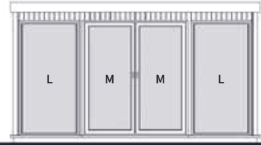
4.27m (14') front with 1.80m double doors
